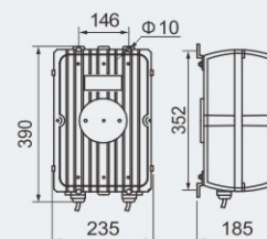
BnT81-1000 Ballast
